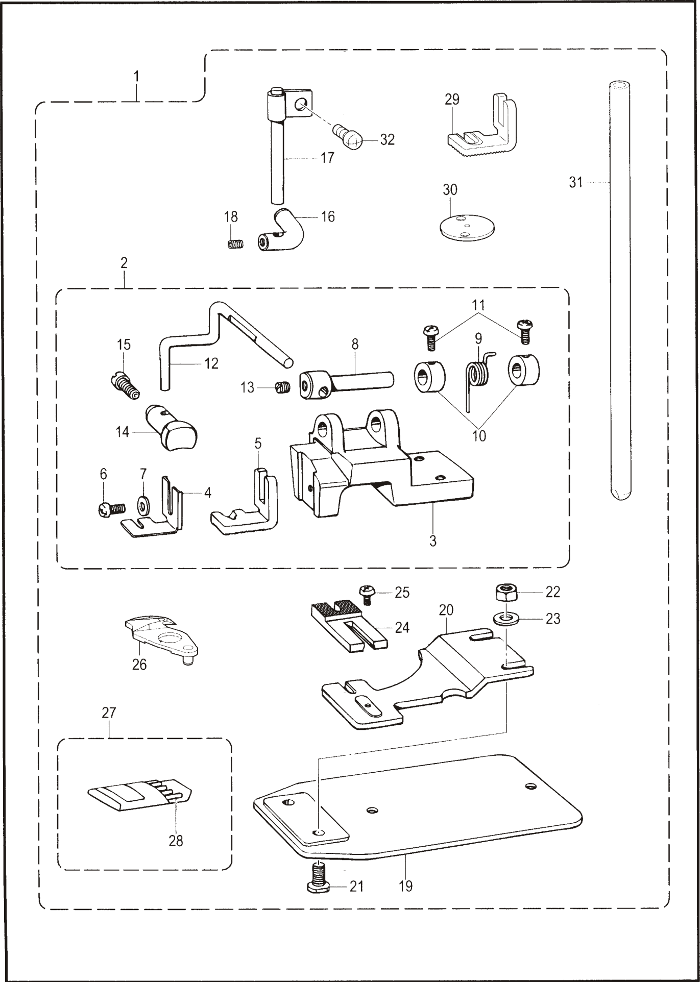
V1. 辅助装置(用于 CSM-438D 的选购零部件) / Auxiliary device (Option parts for CSM-438D)
