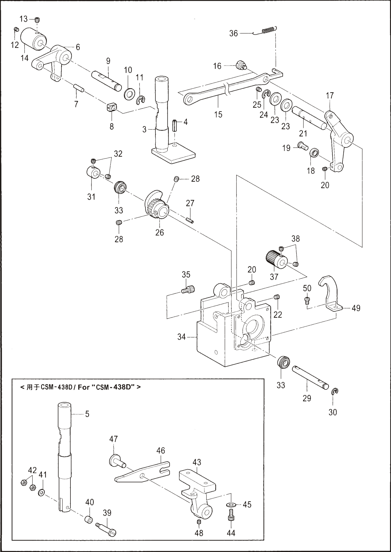
D. 抬压装置 / Work clamp lifter mechanism
